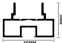
SH-2035 16MM X 45MM TOP & BOTTOM PROFILE (2.8KG/10 FEET)
